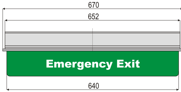
HLP 20-1080/HLP 20-2080
